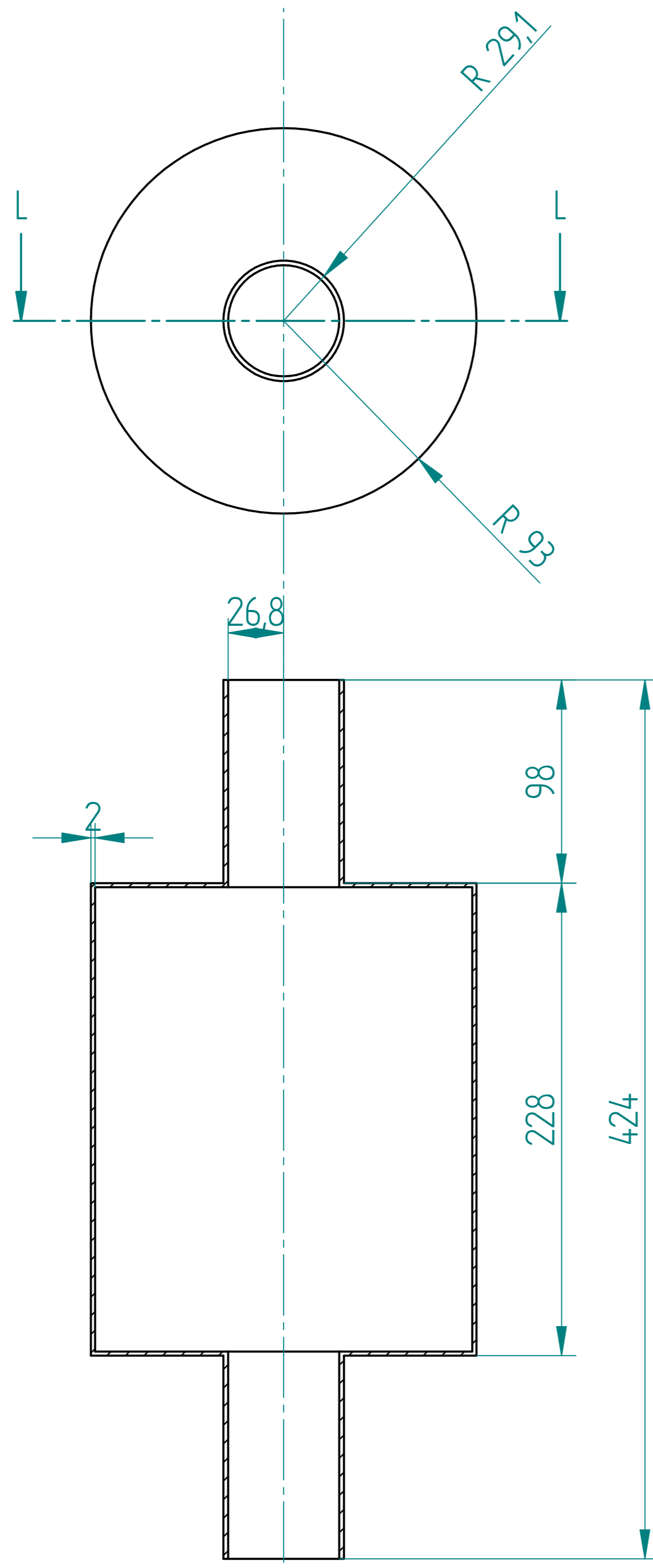
SECTION L-L
